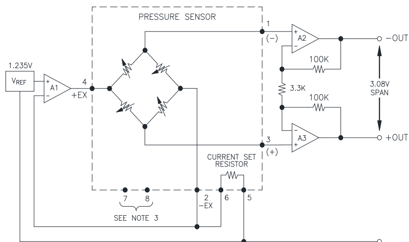
APPLICATION SCHEMATIC
